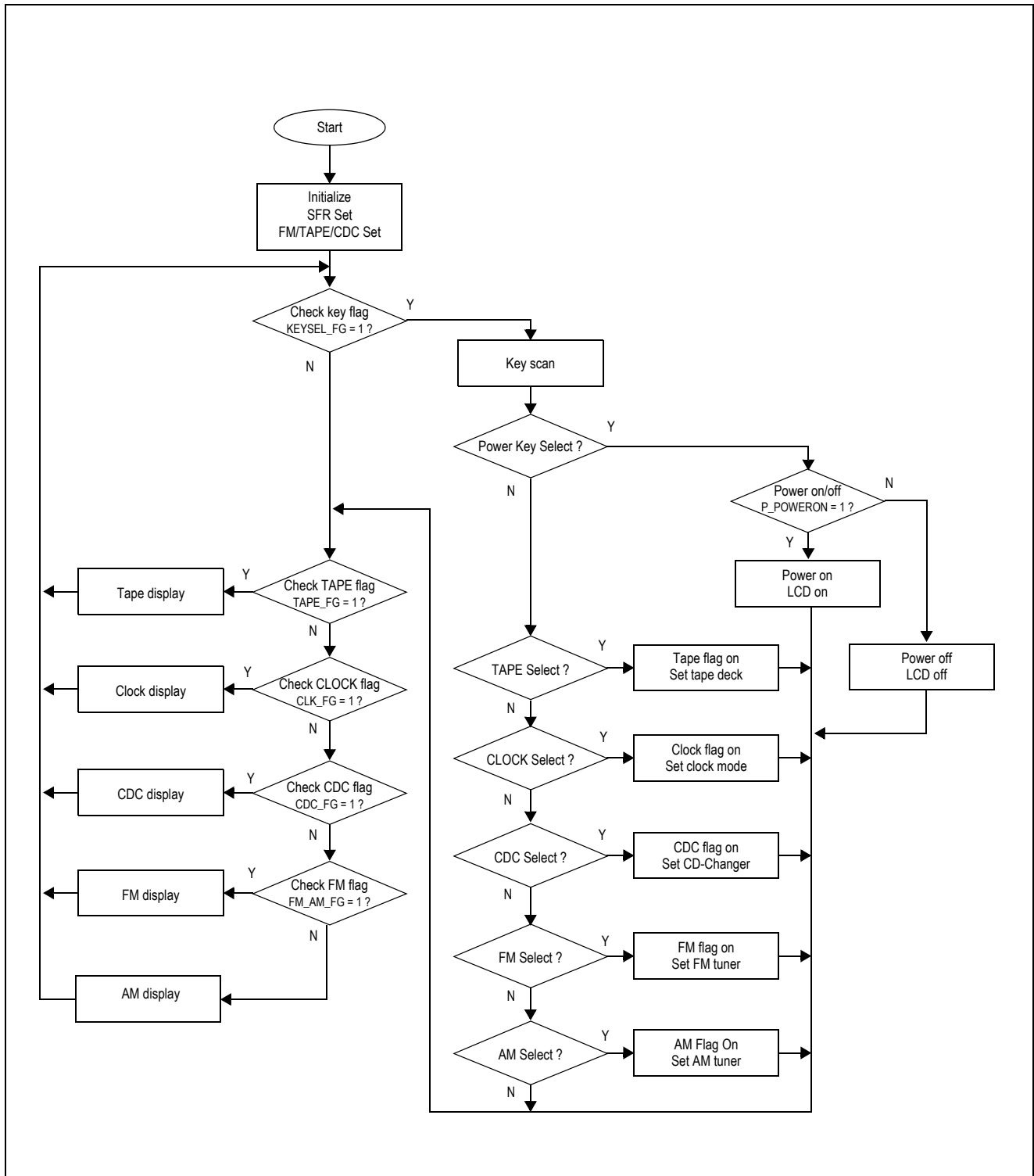
Figure 2. Car Audio System Flow Chart
