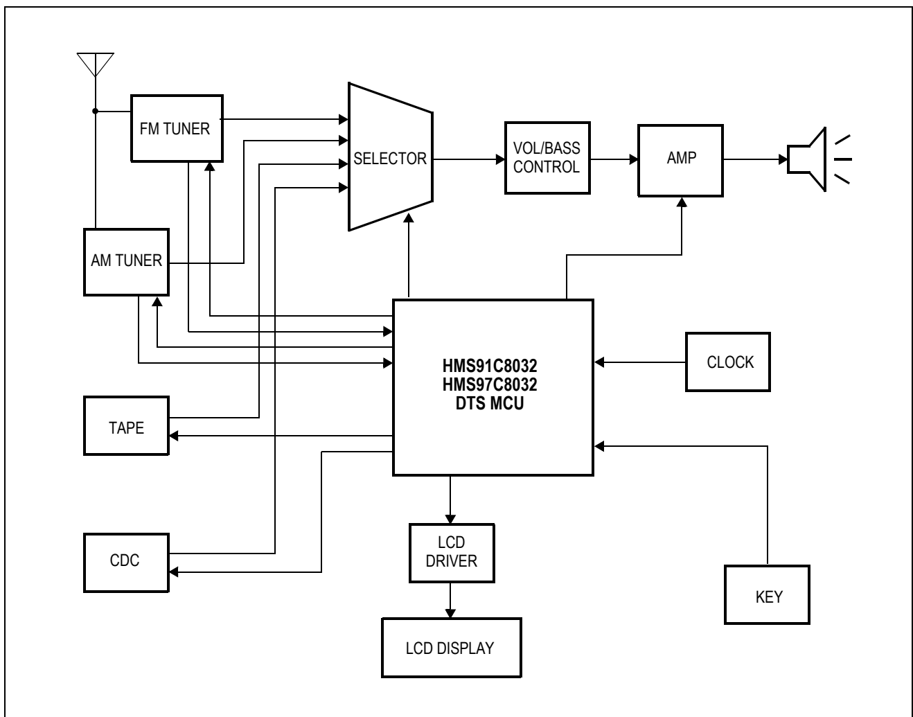
Figure 1. Car Audio System Block Diagram
