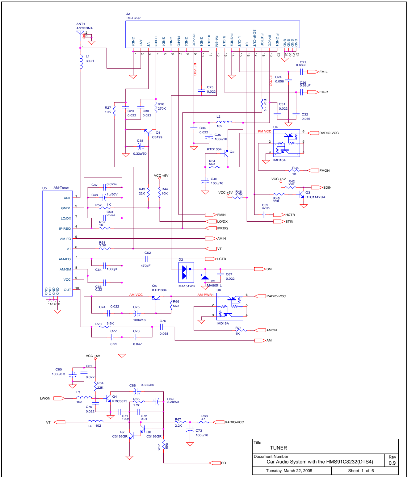
Figure 3. Tuner of Car Audio System
