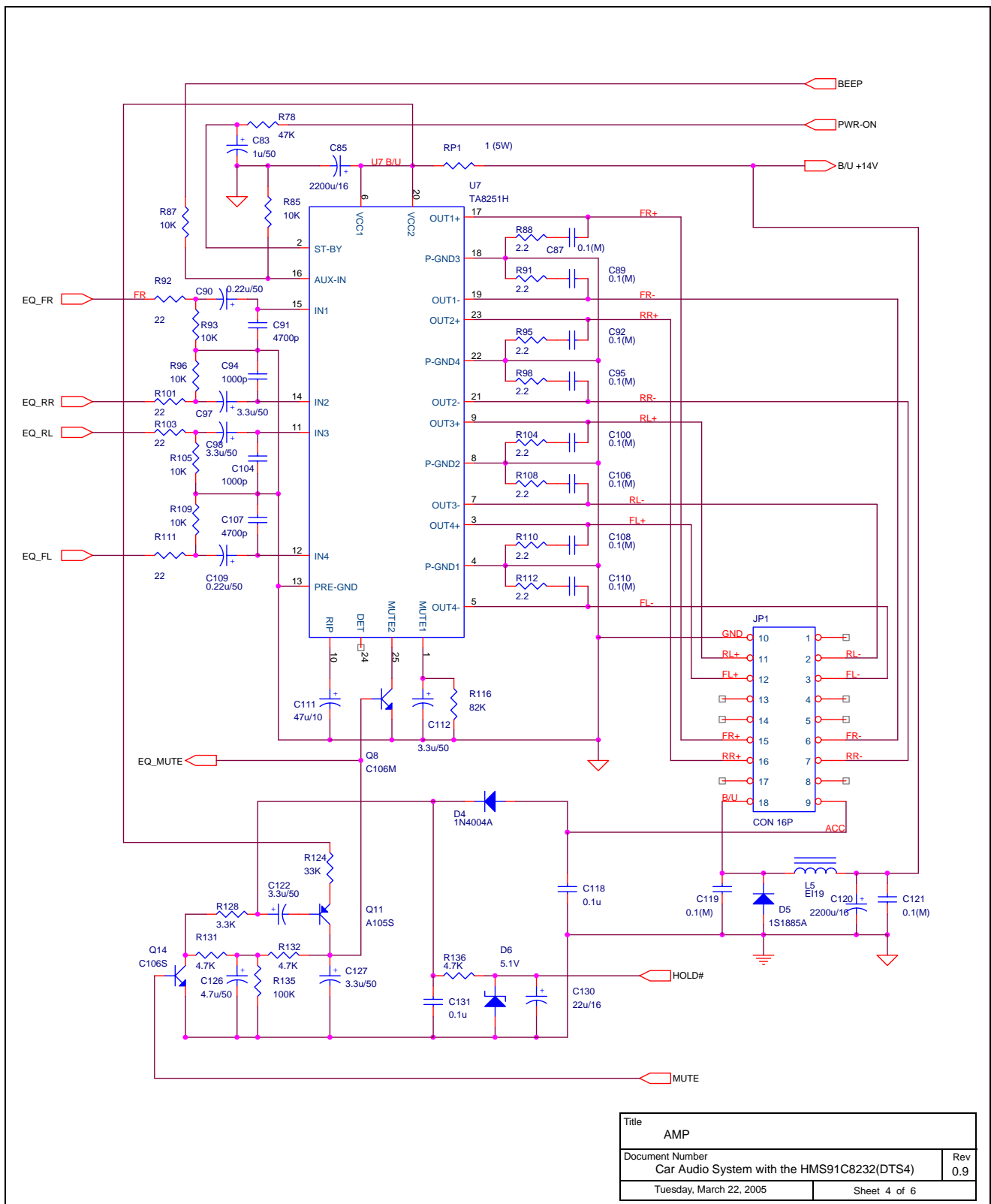
Figure 6. AMP of Car Audio System
