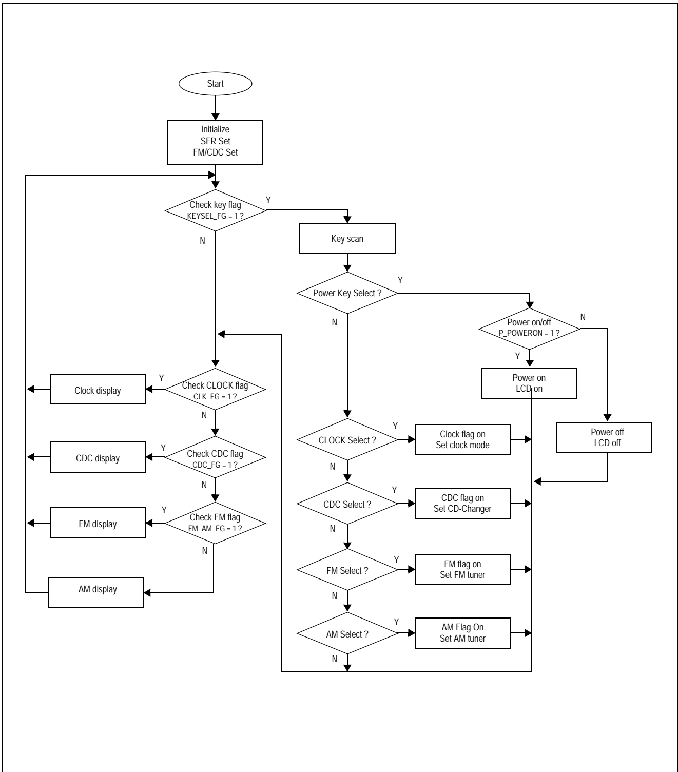
Figure 2. Flow Chart of Car Audio System
