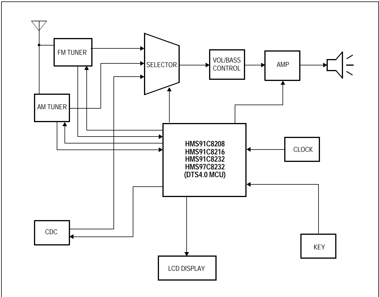
Figure 1. Block Diagram of Car Audio System
