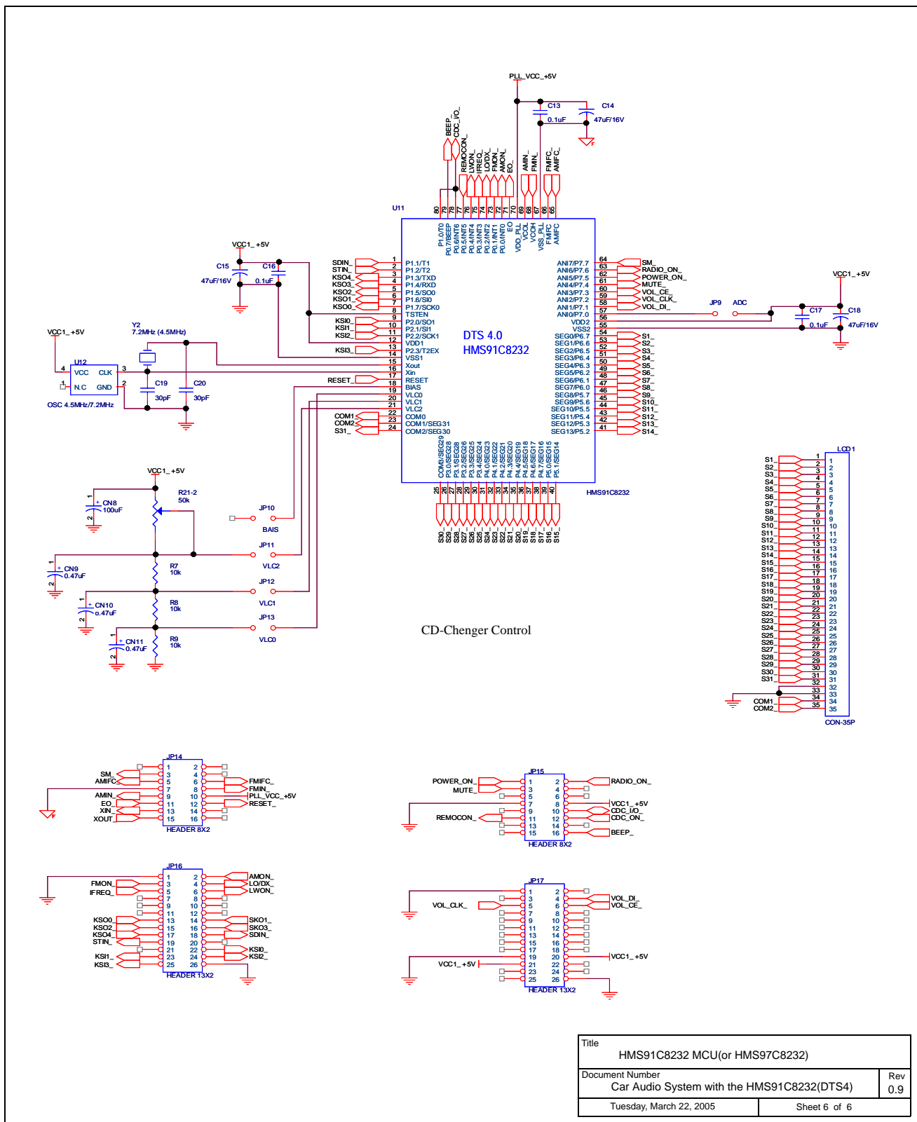
Figure 8. MCU of Car Audio System
