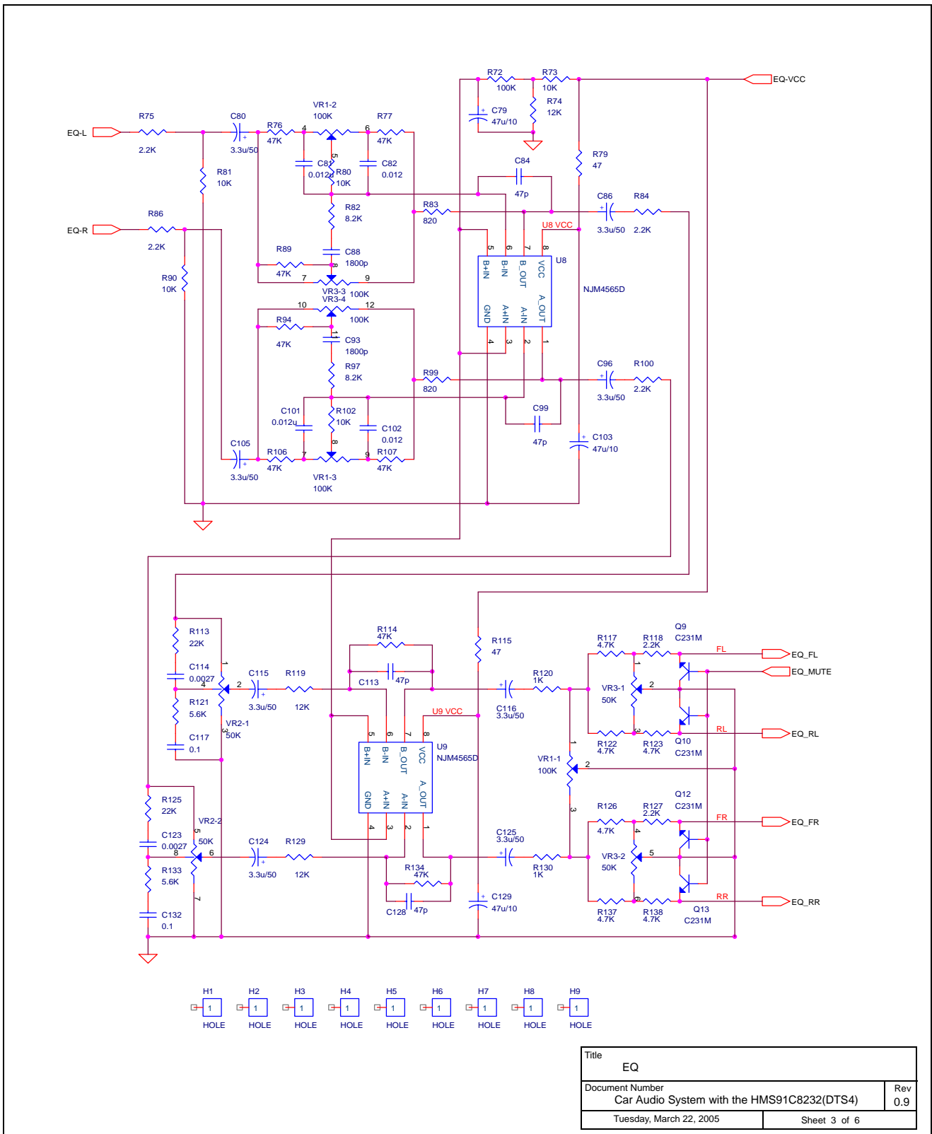
Figure 5. EQ of Car Audio System
