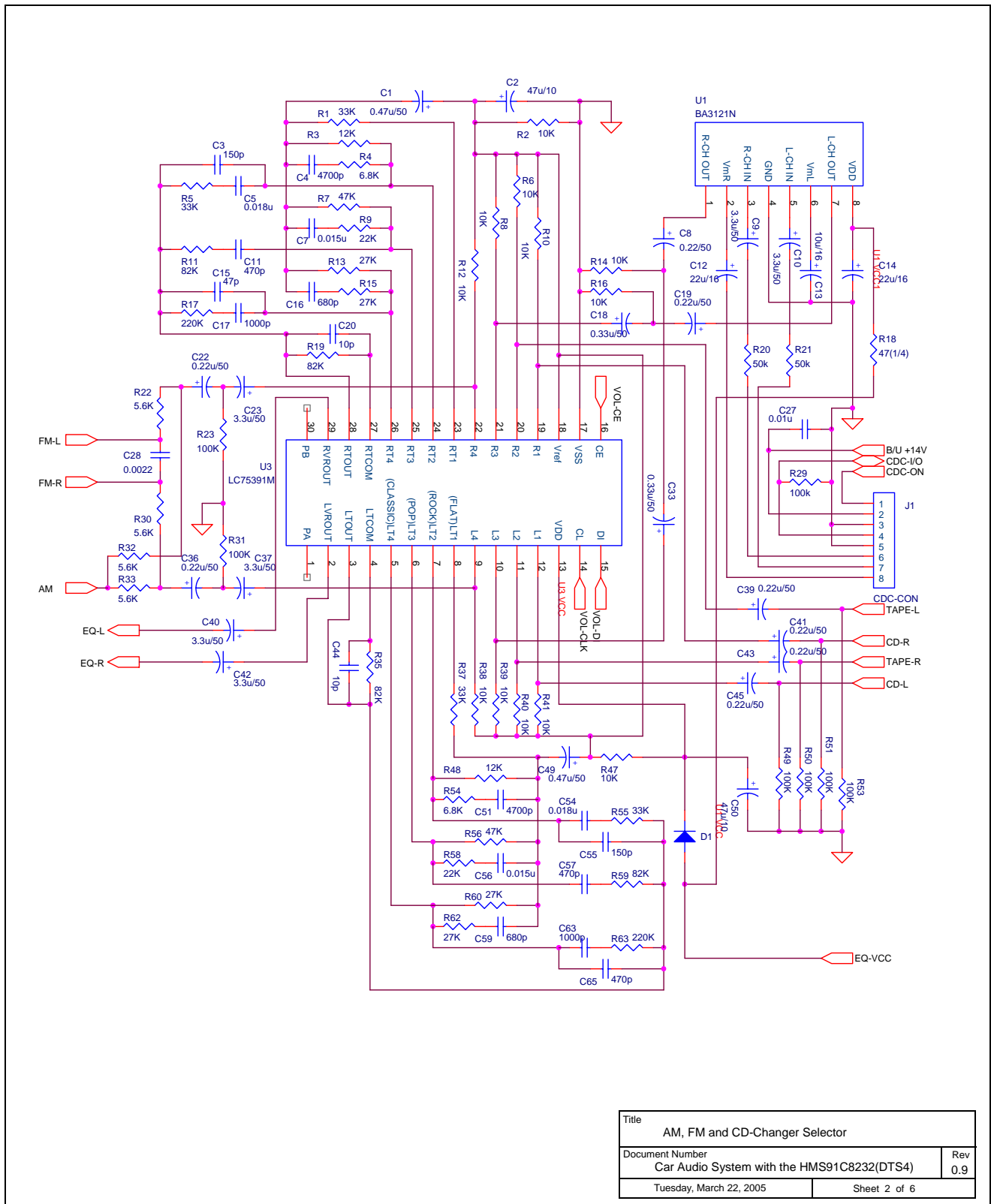
Figure 4. Selector of Car Audio System
